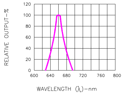
Fig.2 SPECTRAL RESPONSE
